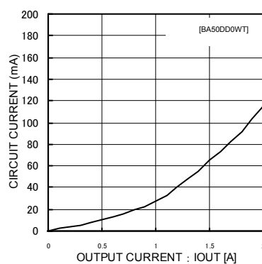
Fig.20 負荷別回路電流 ( I_{out}=0mA \rightarrow 2A )
